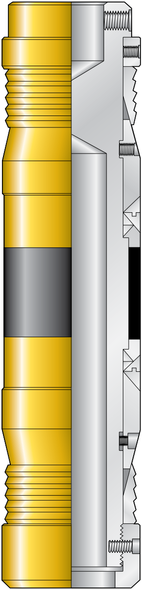
N and N-2 Tubing Size Bridge Plugs Product Family No. H40103
